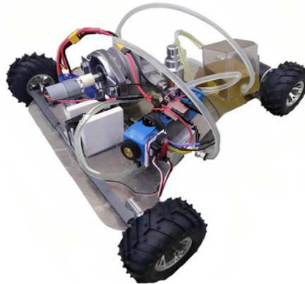
Figure 1. Modular miniature kit for a remote-controlled hydraulic vehicle [11]
