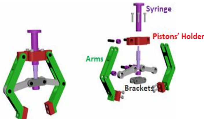
Figure 2. CAD model for a light-duty gripper
